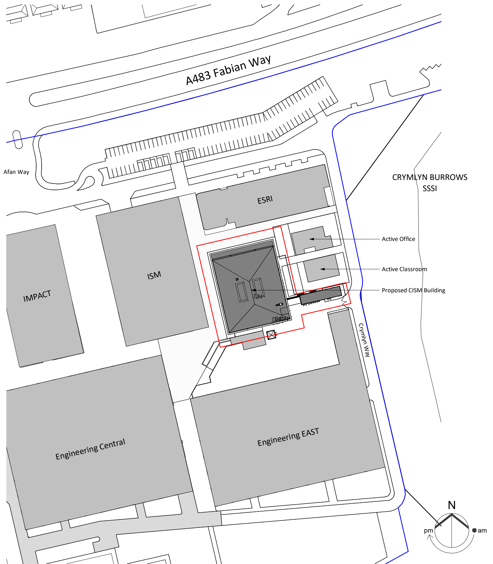
Site Plan. Planning Issue 1 : 1250
